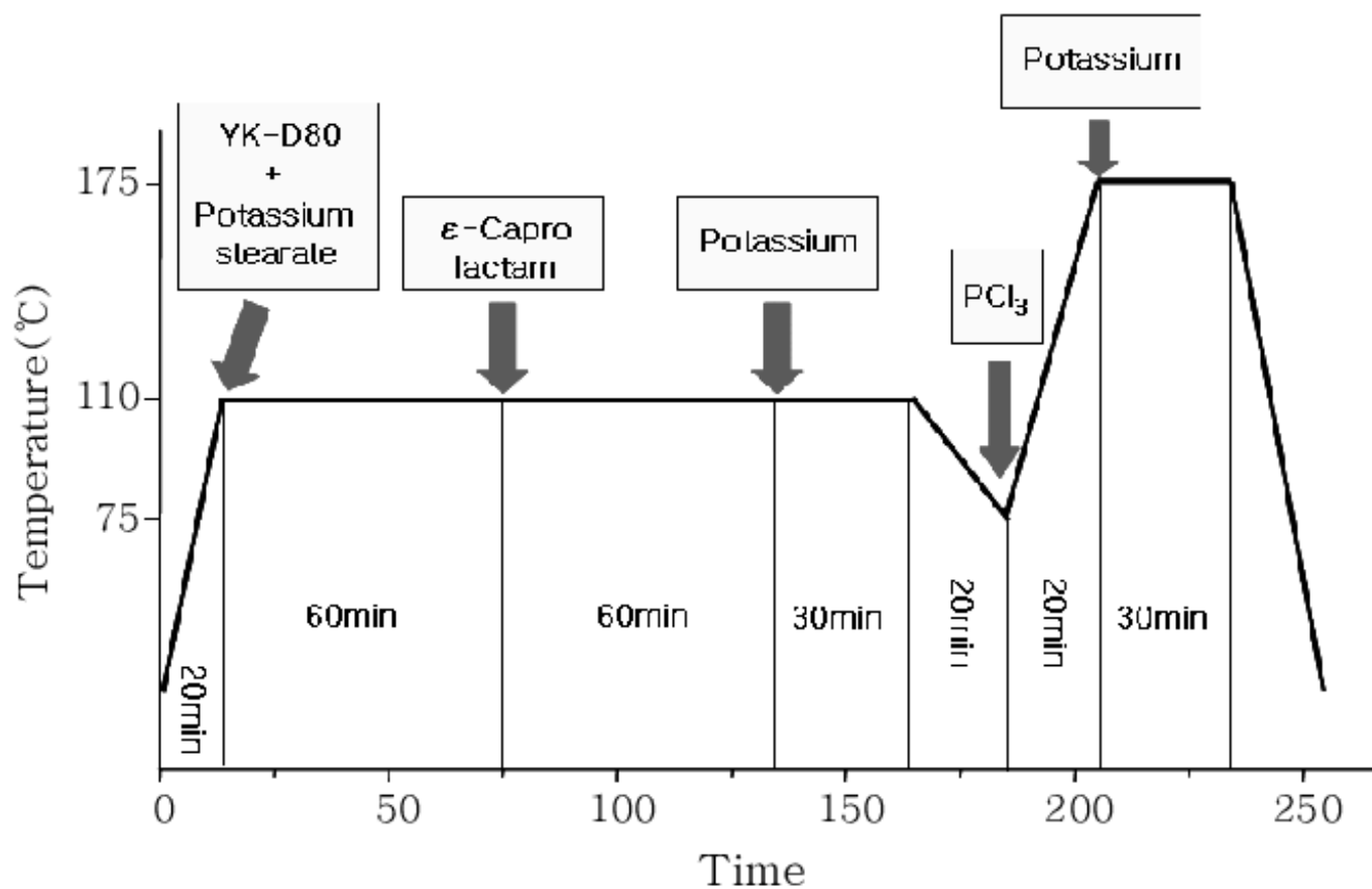
Figure 1 Reaction procedure of polymerization
